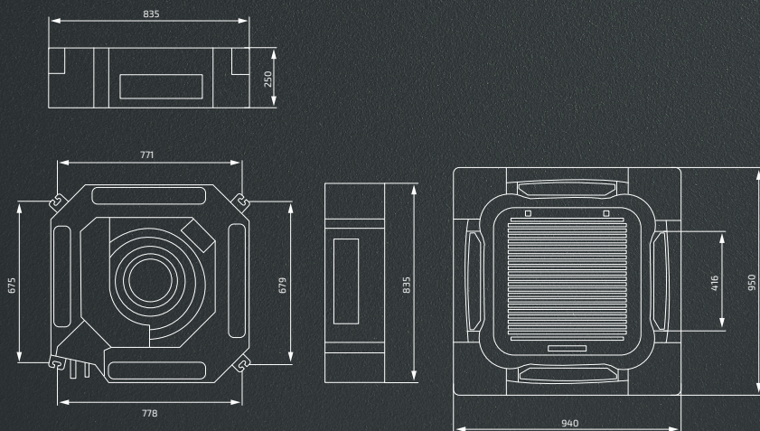
FF60/80C-2PA1
